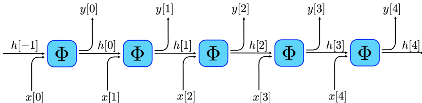
Figure: Unfolded RNN
